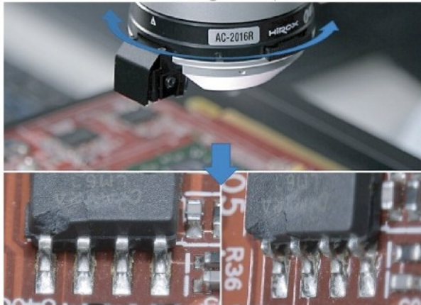
PCB 360 Degree Inspection
